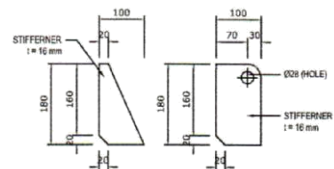
DETAIL STIFFENER PLATE
