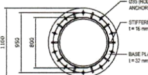
SECTION - A
