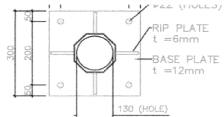
SECTION - A
