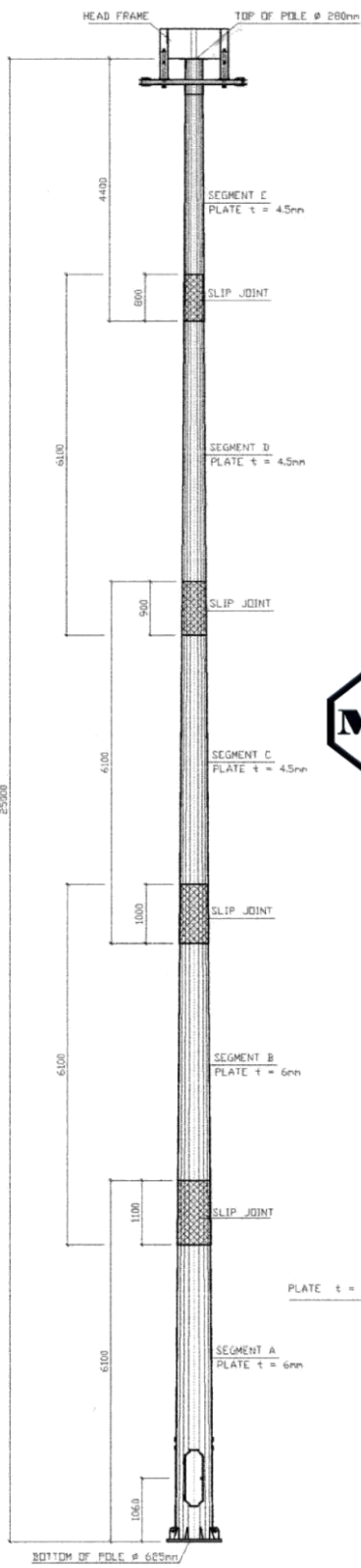
FRONT VIEW
