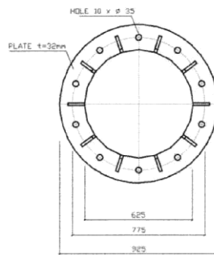
DETAIL BASE PLATE
