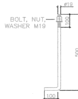
DETAIL ANCHOR BOLT M19
