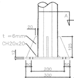
DETAIL 1
