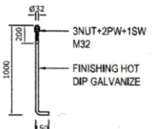
DETAIL ANCHOR BOLT
