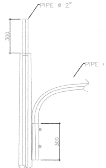
DETAIL 2
